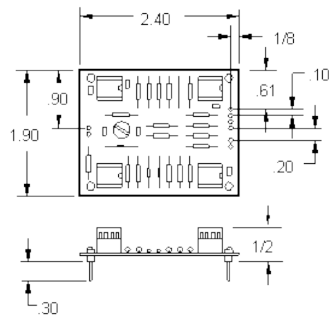
DIMENSIONS:
