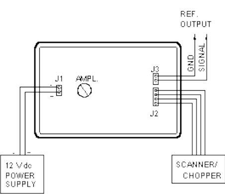
HOOK UP DIAGRAM:
