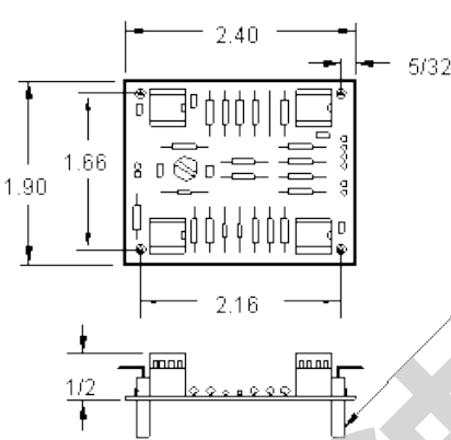
DIMENSIONS:
