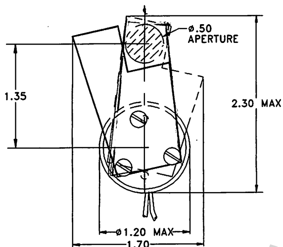
SH-10: OUTLINE DRAWING
