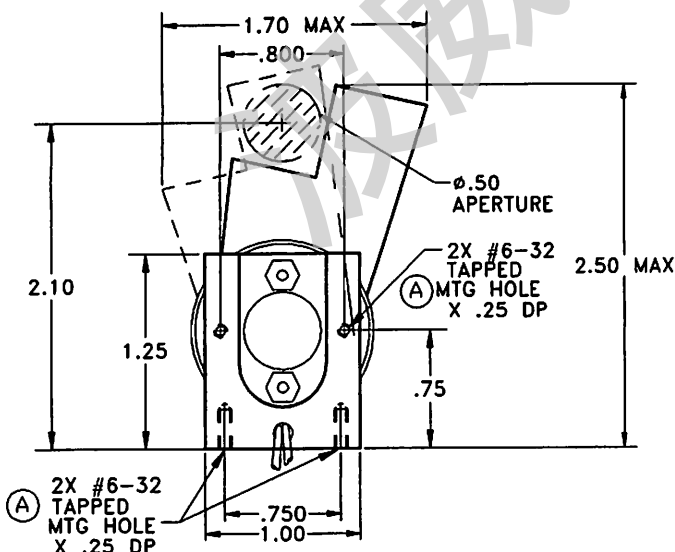
SH-10-M: OUTLINE DRAWING
