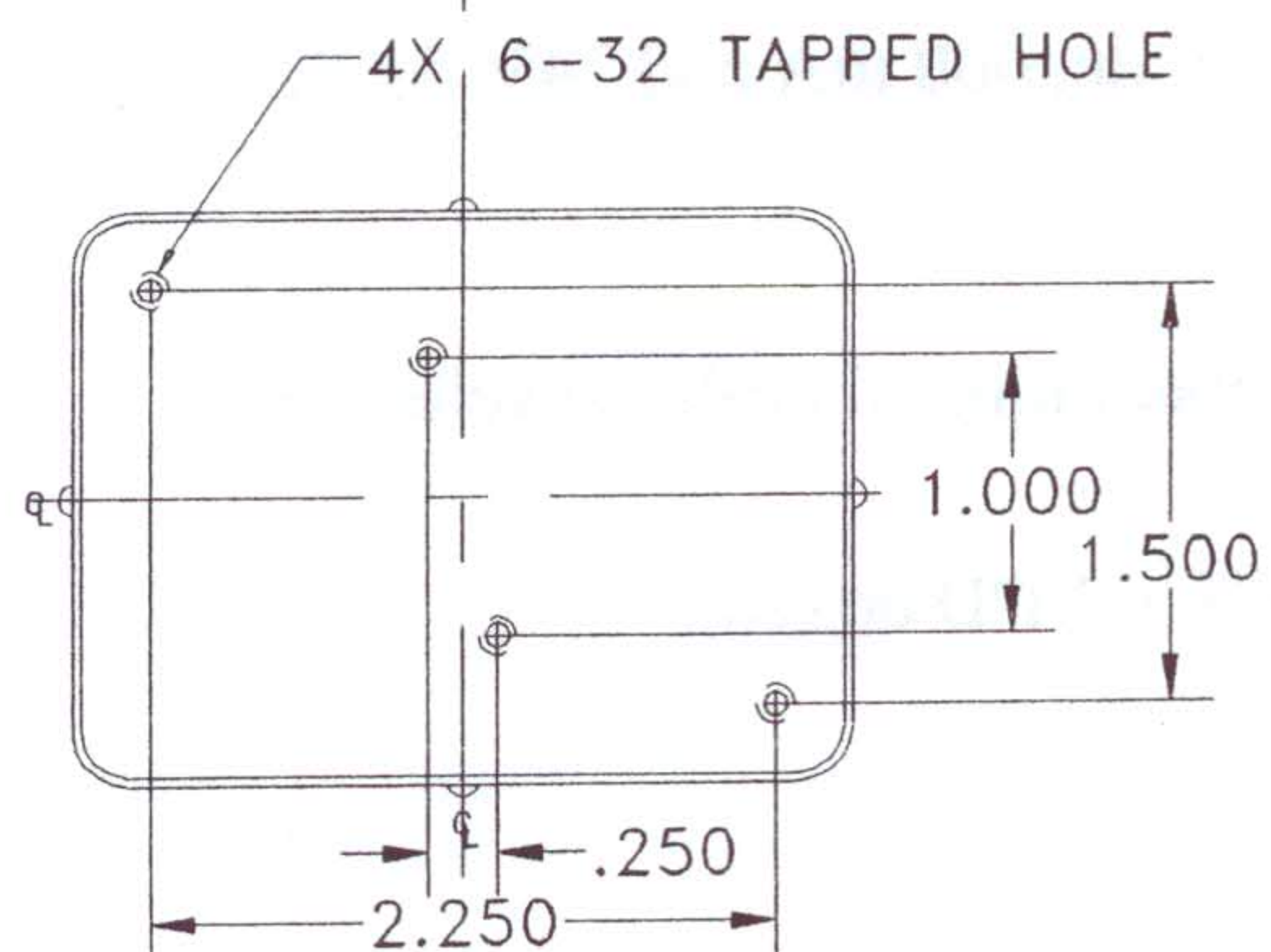
SH-20-B: OUTLINE DRAWING
